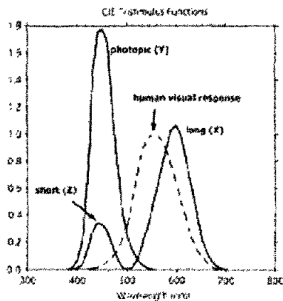
Figure 3. CIE Tristimulus functions
